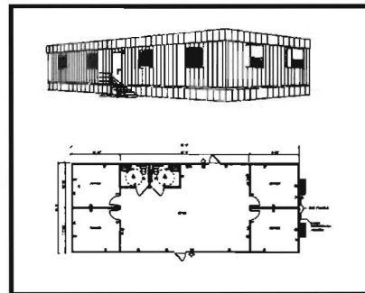
24' x 60' DOUBLE WIDE OFFICE
